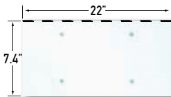
VP120000 HINGED 1 TAG HANGER 18 GA. STAINLESS PETE 389
